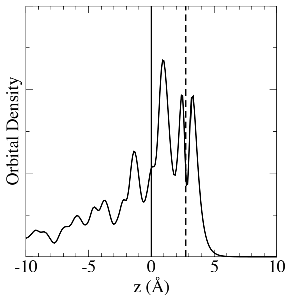
FIG. 4. Orbital density of the FE band at the \Gamma point of the SBZ as a function of the coordinate z perpendicular to the surface. The density has been laterally averaged and the vertical solid line gives the average position of the first layer of Ag atoms. The average position of the perylene core is indicated by the vertical dashed line.
