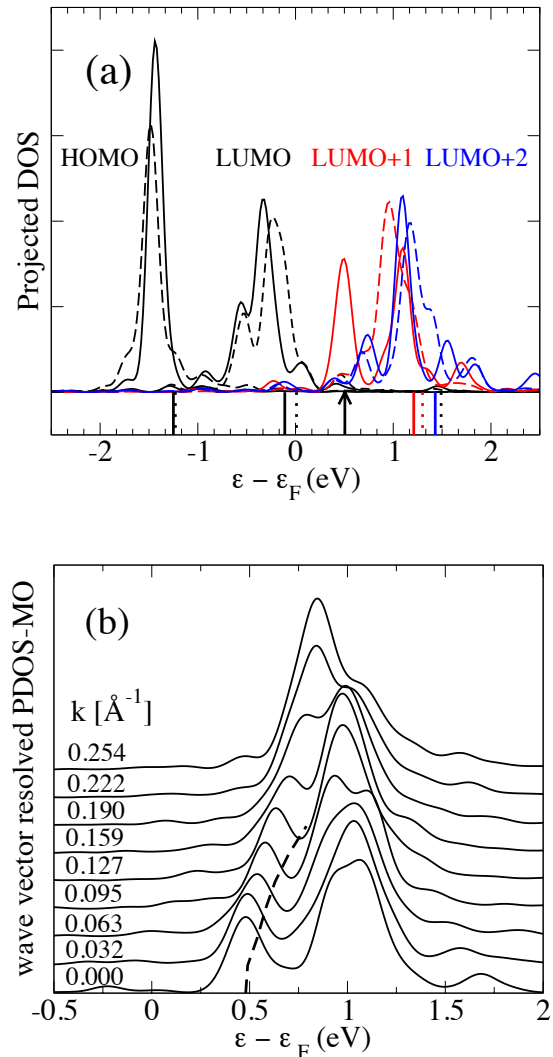
FIG. 1. Projected DOS (PDOS) of the adsorbed PTCDA monolayer on the frontier molecular orbitals of the isolated PTCDA monolayer. In (a) PDOS on the HOMO, LUMO, LUMO+1, and LUMO+2 are taken at the \Gamma point in the SBZ. The dashed and solid lines correspond to the projected DOS of the two nearly degenerate MOs of the two molecules in the surface unit cell. Their energies when aligning the vacuum levels of the isolated and the adsorbed monolayer are indicated by vertical bars. The vertical arrow indicates the position of the satellite peak in one of the LUMO+1 states. The dispersion of the projected DOS on the LUMO+1 is shown in (b) where the dashed line indicate the energies of the peak positions in the PDOS. Both LUMO+1 states are included in (b).
