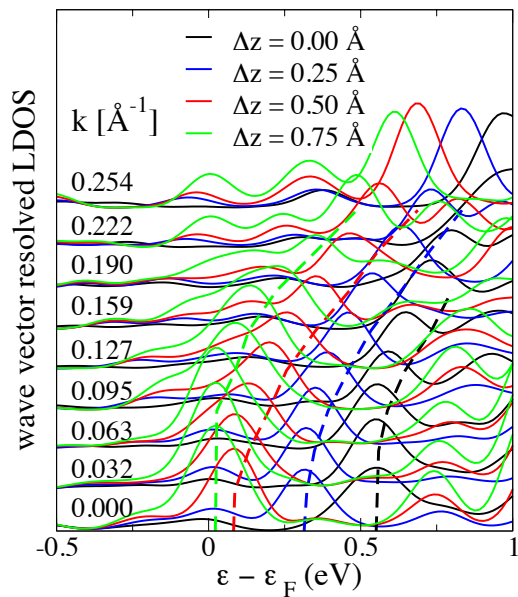
FIG. 5. Evolution of wave vector resolved LDOS of the PTCDA monolayer adsorbed on the Ag slab with the height \Delta z of the monolayer from its equilibrium position on the surface. The magnitude k of the parallel momentum along the direction in the surface Brillouin zone boundary is indicated and k = 0.254 Å -1 corresponds to the zone boundary. The thick dashed lines indicate the energies of the peak positions in the LDOS. The states were broadened by 0.1 eV.
