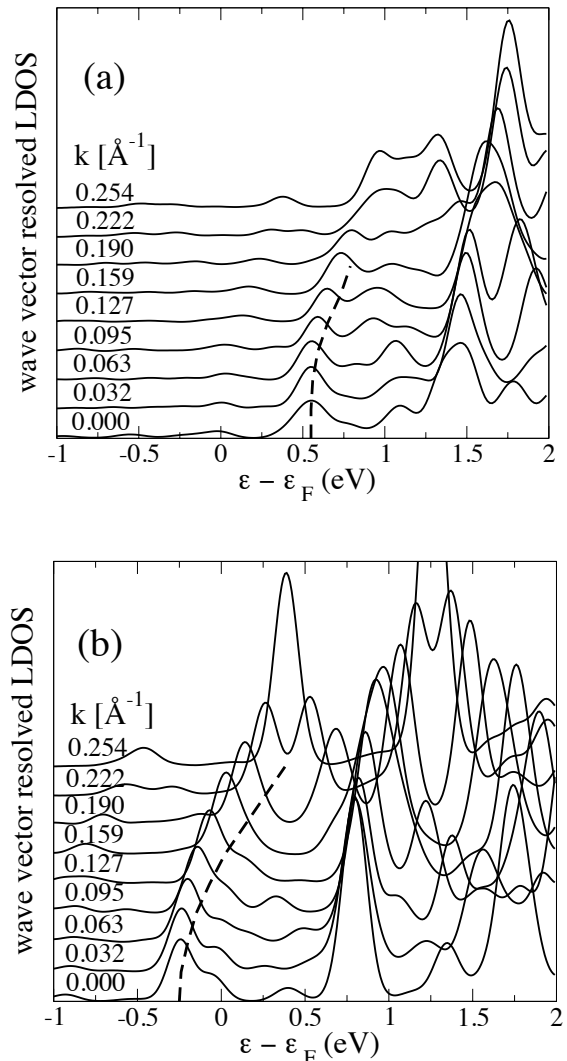
FIG. 2. Wave vector resolved LDOS of the PTCDA monolayer adsorbed on the Ag slab (a) and the bare side of the Ag slab (b) at distance of 7 Å from the top Ag layer. The magnitude k of the parallel momentum along the direction in the surface Brillouin zone boundary is indicated and k = 0.254 \text{ \AA}^{-1} corresponds to the zone boundary. The thick dashed lines indicate the energies of the peak positions in the LDOS. The states were broadened by 0.1 eV.
