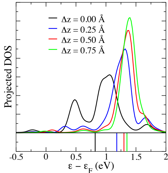
FIG. 6. Evolution of the projected DOS (PDOS) of the adsorbed PTCDA monolayer on the LUMO+1 with the height \Delta z of the monolayer from its equilibrium position on the surface. The projection is taken at the \Gamma point in the SBZ and both LUMO+1 states are included. The average energies of the PDOS are indicated by vertical bars. The states were broadened by 0.1 eV.
